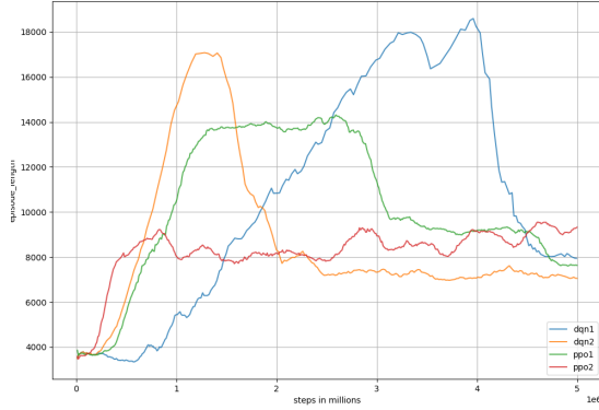
Fig. 4. Episode Length Training Phase Result
